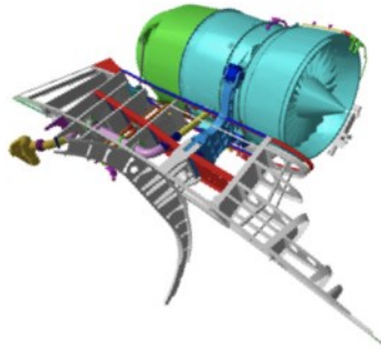
Figure 1. Pylon example
