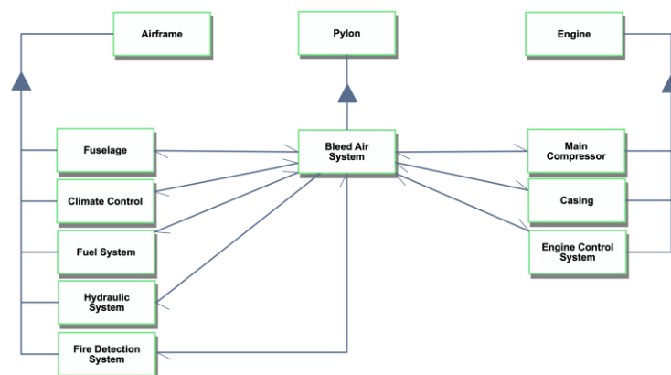
Figure 7. Bleed Air System interfaces representation in OPM
