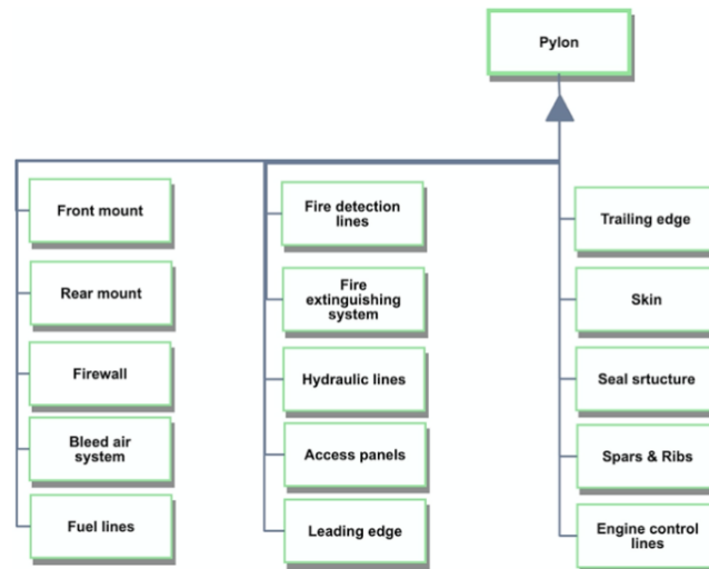
Figure 3. Pylon decomposition
